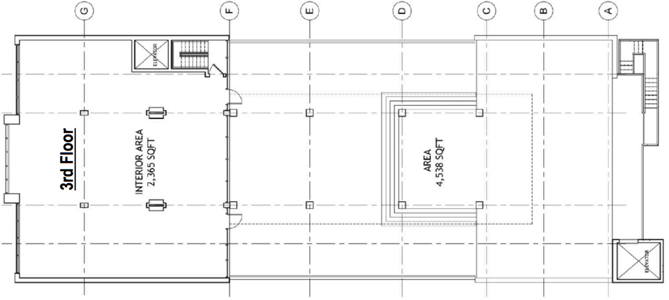
3) THIRD FLOOR PLAN - CONCEPT 1/8" = 1'-0"
