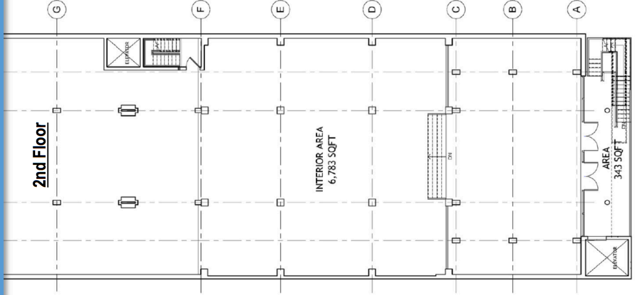
2) SECOND FLOOR PLAN - CONCEPT 1/8" = 1'-0"
